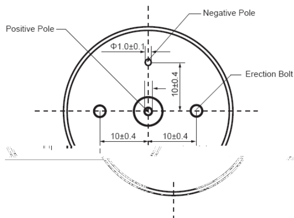
THC2W \Phi 36 \times 12/16 outline (A) Unit:mm
