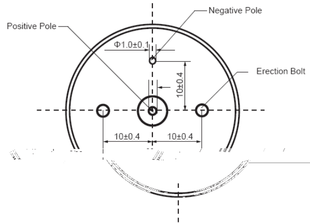
THC2W \Phi 36 \times 12/16 outline (B) Unit:mm
